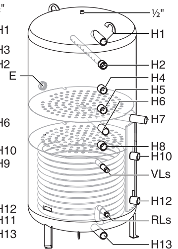
BHS 750, 1000-6 ERZ
